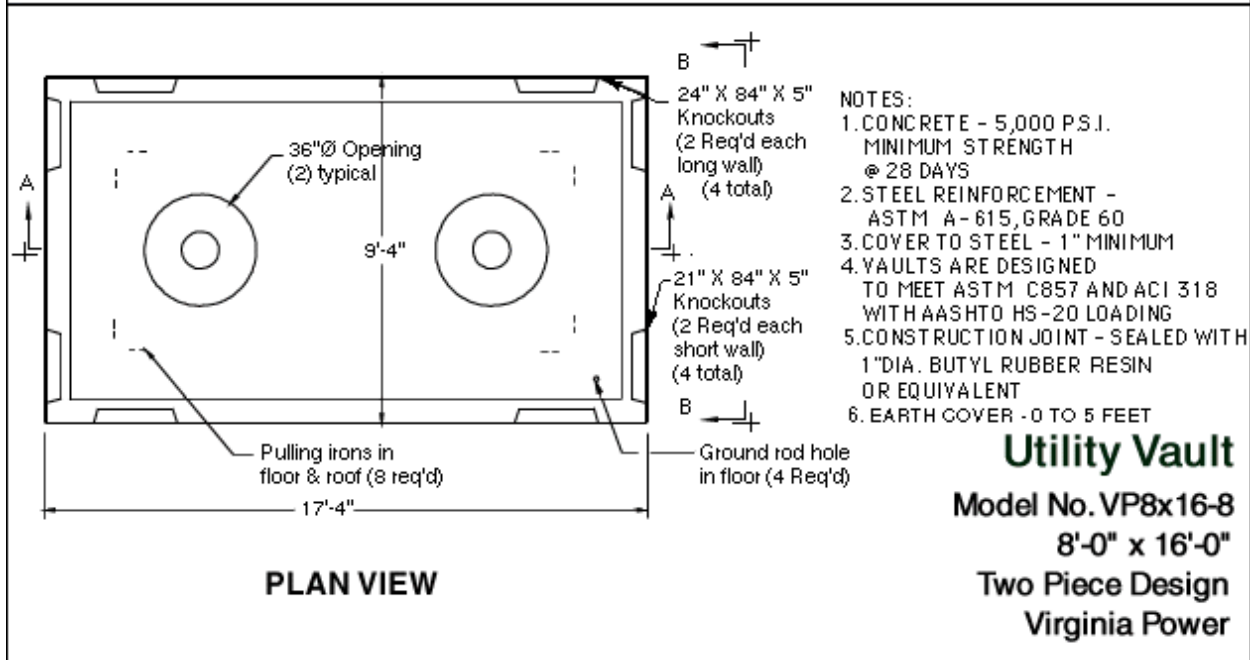
Utility Vault Model No. VP8x16-8 8'-0" x 16'-0" Two Piece Design Virginia Power
