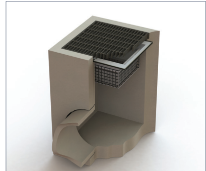
Flat-Grated Inlet
