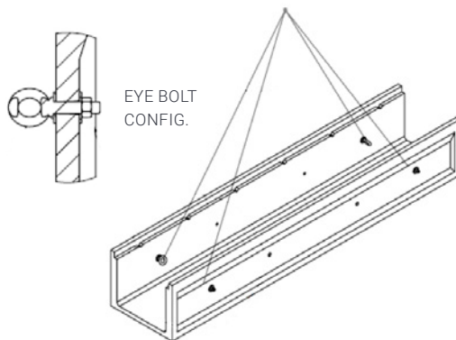
Preferred Method: Eye Bolt
