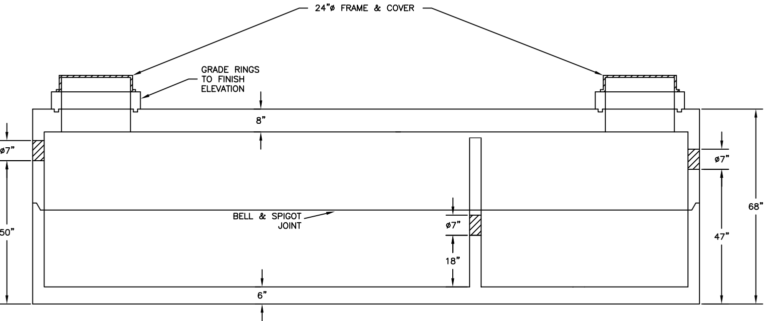
SECTION VIEW
