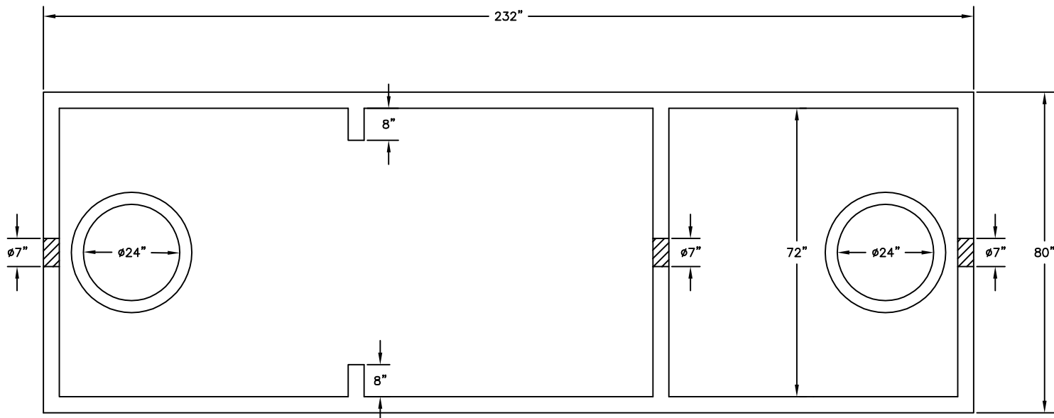
PLAN VIEW
