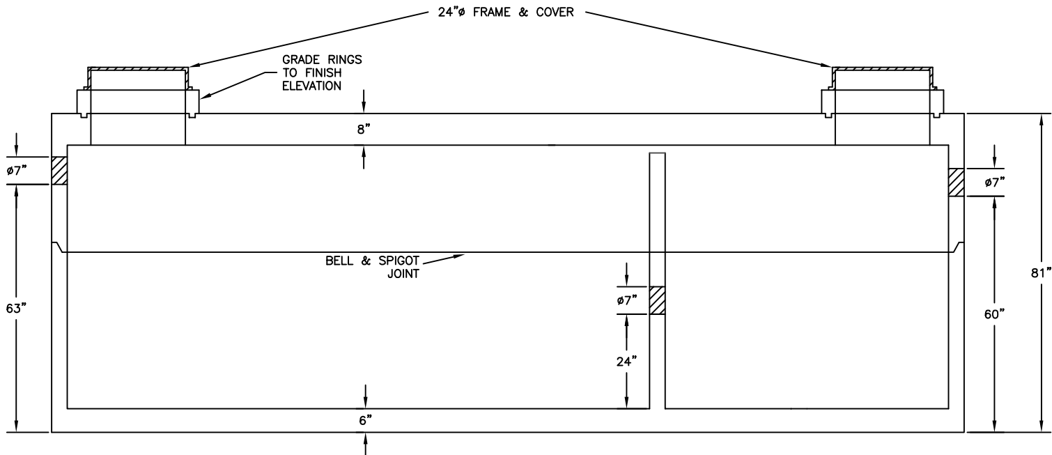
SECTION VIEW
