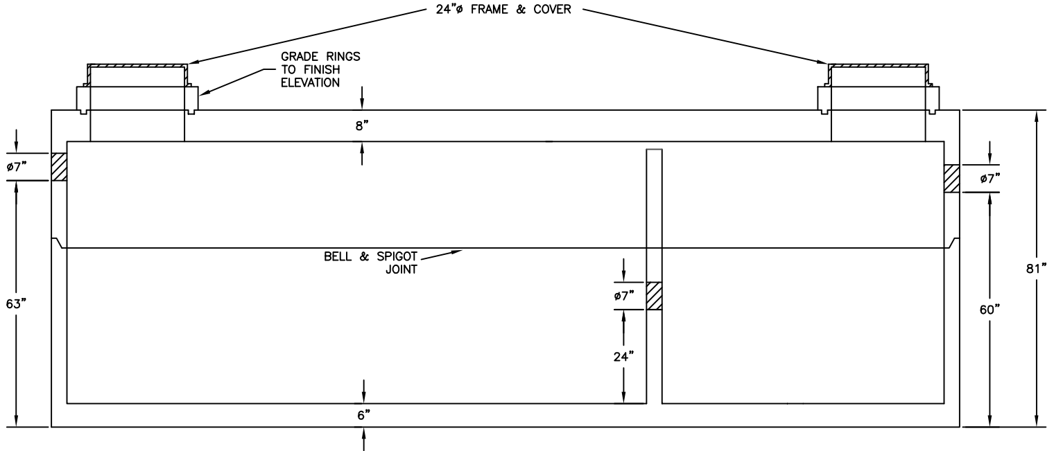
SECTION VIEW
