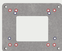
CMP-003 3048 Cabinet Mounting Plate for ● Clearfield FieldSmart FDH 144, 288, 432 PON ● Clearfield FieldSmart FDH 432 Cross Connect ● Comscope 144 ● Corning Gen III
