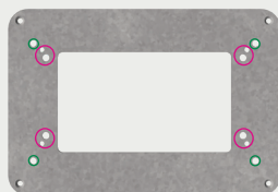
CMP-001 3660 Cabinet Mounting Plate for ● Inventronics BC48X18 ● ADC 3000 FDH
