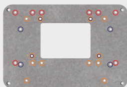
CMP-022 3660 Cabinet Mounting Plate for ● Clearfield FieldSmart FDH 144, 288, 432 576 PON ● Clearfield FieldSmart FDH 432, 864 Cross Connect ● Comscope 144, 288, 432, 576 ● Corning Gen III ● Corning LS 144, 288, 432
